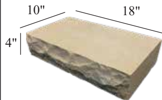
24" CHAMFER CAP
